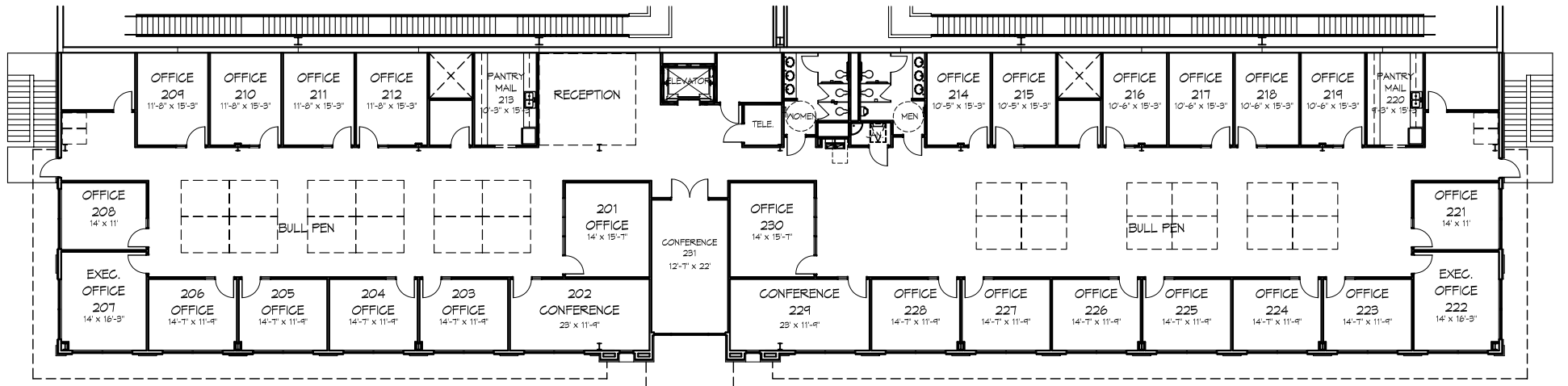
SECOND FLOOR - 11,983 SF
